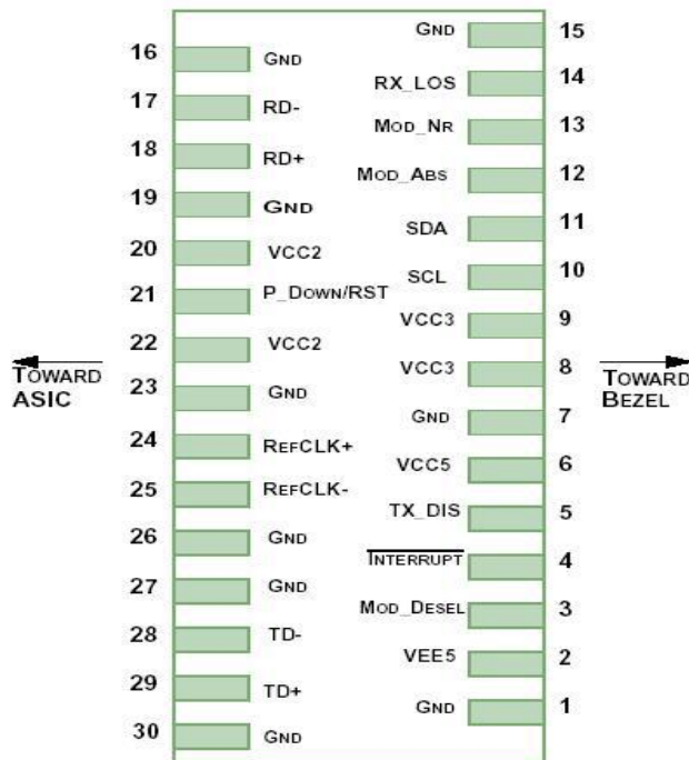
Figure1.Electrical Pin-out Details
